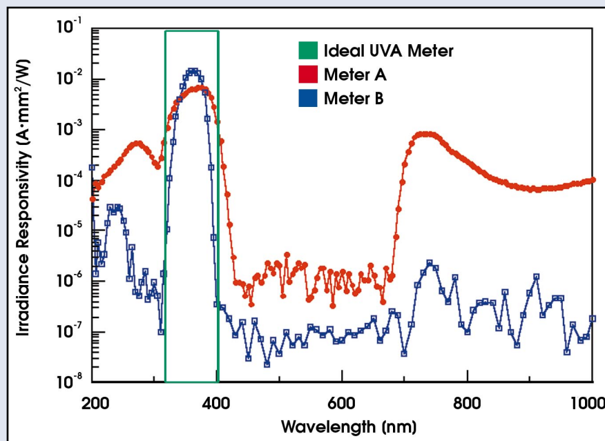
Figure 2. The spectral responsivity differs between two broadband UV meters used in semiconductor photolithography to determine the total exposure of a photoresist to 365-nm radiation from a filtered mercury source. 5 The graph also points out the spectral responsivity of an "ideal" UVA meter.
