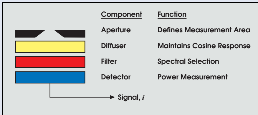
Figure 1. A UV radiometer comprises a number of relatively simple optical elements.
