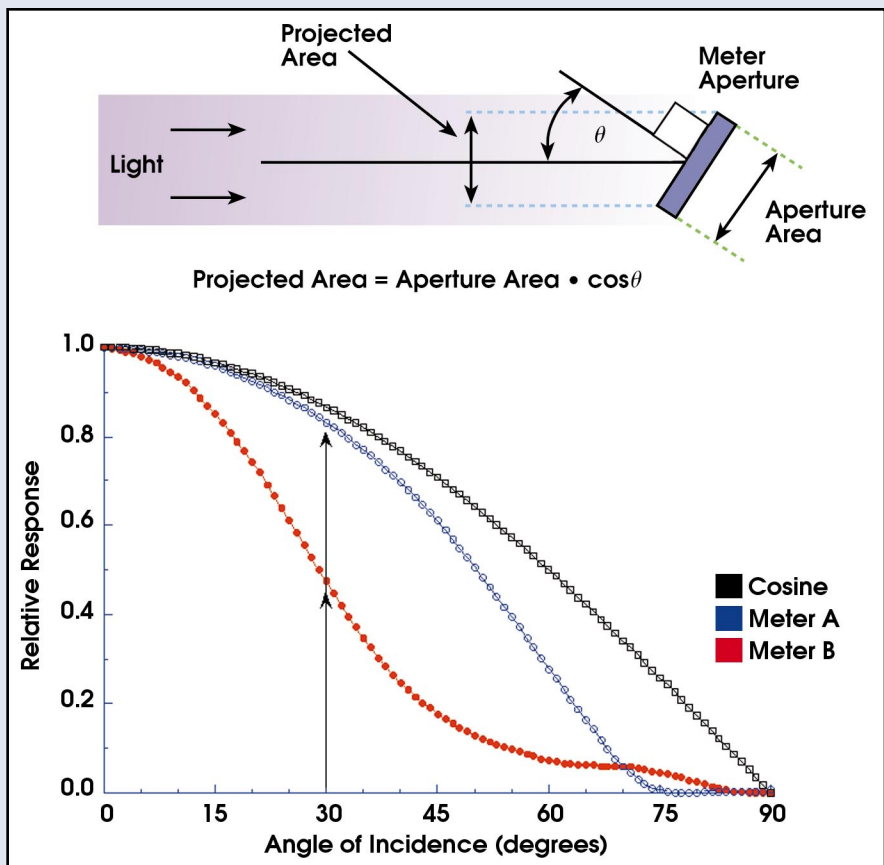
Figure 4. Two UV meters' angular responses differ not only from each other, but also from an ideal cosine response. Meter A's responsivity to light 30° from normal was 3.5 percent less than ideal, and Meter B's was 45 percent less. The inset shows the geometry illustrating how angle affects the signal measured by a meter.
