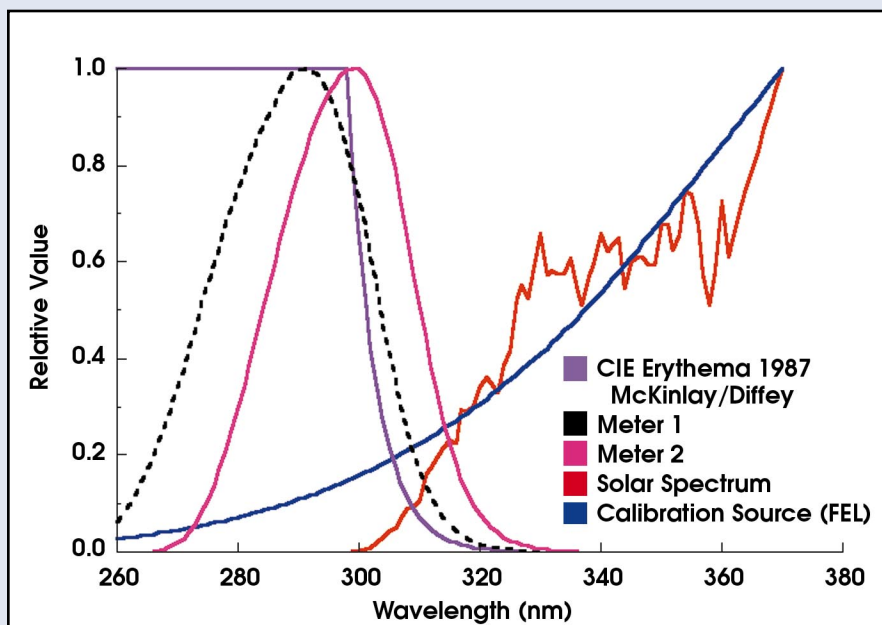
Figure 5. Two UV radiometers exhibit a mismatch to the CIE 1987 erythema function. 7 This shows the uncertainties that can arise when the calibration source differs from the measurement source.
